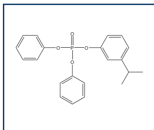
3IPDP
